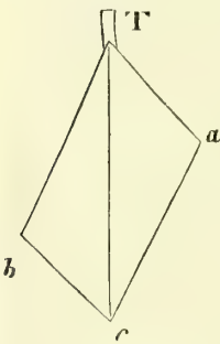
Composition of Forces.
